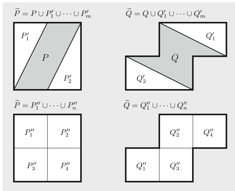
For a parallelogram P and a nonconvex hexagon Q that are equicomplementary, this figure illustrates the four decompositions we refer to.
