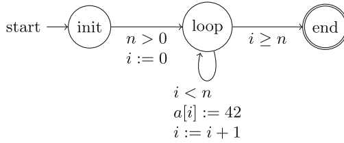
Fig. 1. Compact control-flow graph for Program 1
