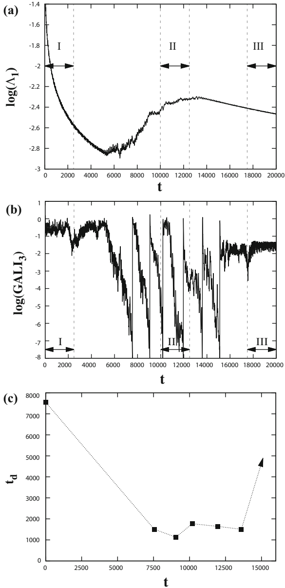
Fig. 5.23 Time evolution of (a) the finite time mLE \Lambda_1 , (b) the re-initialized \text{GALI}_3 , and (c) the time t_d needed for the re-initialized \text{GALI}_3 to decrease from \text{GALI}_3 = 1 to \text{GALI}_3 \leq 10^{-8} for a particular orbit of the 3D time dependent galactic model studied in [68]. The orbit changes its dynamical nature from regular to chaotic and again to regular. Three characteristic epochs are located between the vertical dashed gray lines in (a) and (b) and are denoted by I (regular), II (chaotic) and III (regular). The arrow at the right end of (c) indicates that after t \gtrsim 15,000 the \text{GALI}_3 in (b) does not fall back to zero (until of course, the final integration time t = 20,000 ), which is a clear indication that in this time interval the orbit is regular (after [68])
