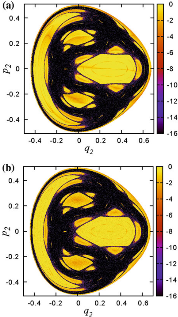
Fig. 5.19 Regions of different values of the GALI_2 on the Poincaré surface of section defined by q_1 = 0 of the 2D Hamiltonian (5.4) for H_2=0.125 . A set of approximately 350,000 equally spaced initial conditions on the grid (q_2, p_2) \in [-0.5, 0.7] \times [-0.5, 0.5] is used. White regions correspond to forbidden initial conditions. The color scales shown at the right of the panels are used to color each point according to the orbit's \log(GALI_2) value at t = 2000 . In (a) the same set of initial orthonormal deviation vectors was used for the computation of the GALI_2 of each initial condition, while in (b) a different, randomly produced set of vectors was used for each orbit
