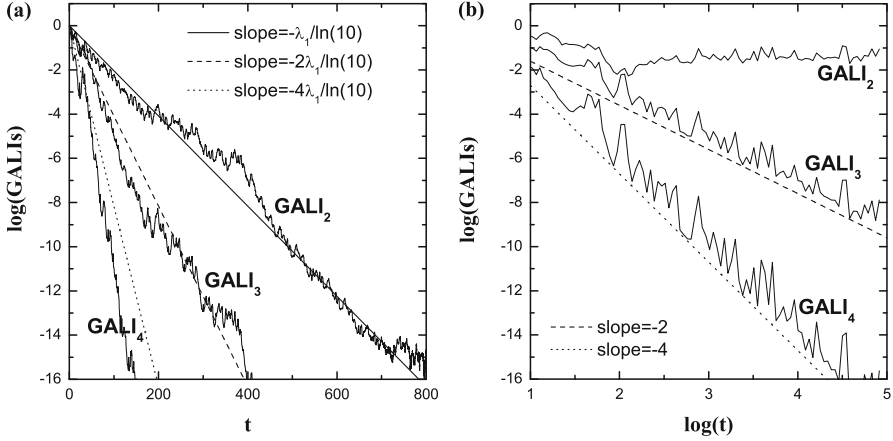
Fig. 5.5 The time evolution of the GALI_2 , the GALI_3 and the GALI_4 for (a) a chaotic and (b) a regular orbit of the 2D Hamiltonian (5.4) for H_2 = 0.125 . The chaotic orbit is the one considered in Fig. 5.3a, while the initial conditions of the regular orbit are q_1 = 0 , q_2 = 0 , p_1 = 0.5 , p_2 = 0 . The straight lines correspond in (a) to functions proportional to \exp(-\lambda_1 t) , \exp(-2\lambda_1 t) and \exp(-4\lambda_1 t) , for \lambda_1 = 0.047 and in (b) to functions proportional to t^{-2} and t^{-4} . The slope of each line is mentioned in the legend. Note that the horizontal, time axis in (a) is linear, while in (b) is logarithmic (after [84])
