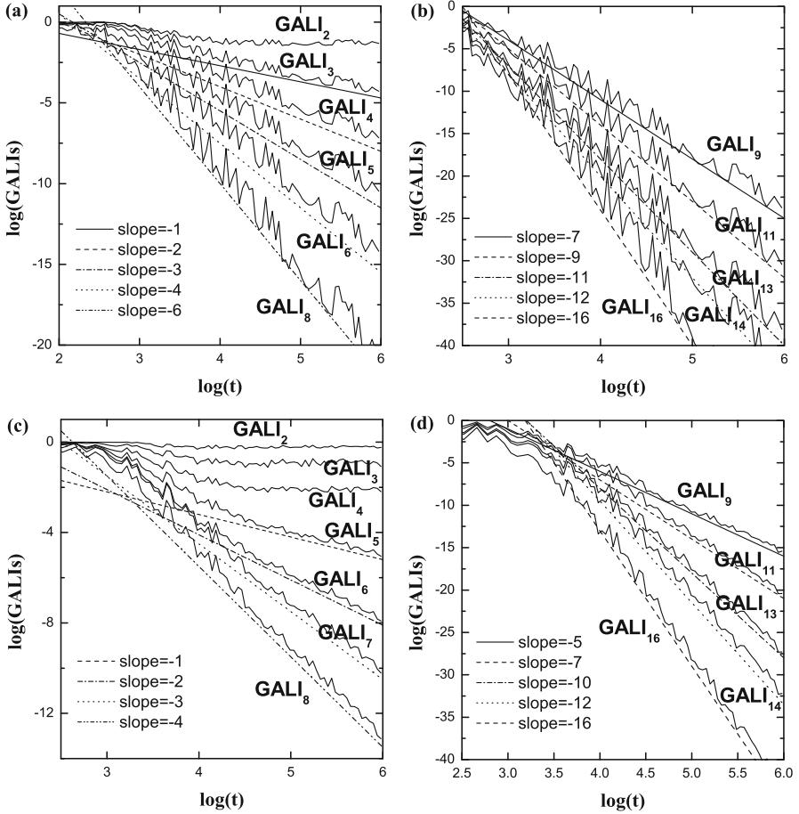
Fig. 5.11 The time evolution of the GALI_k , k = 2, \dots, 9, 11, 13, 14, 16 for a regular orbit lying on a 2d torus (panels (a) and (b)) and for another one lying on a 4d torus (panels (c) and (d)) of the 8D Hamiltonian H_8 considered in Fig. 5.7. The initial conditions of the first orbit are Q_1 = 2 , P_1 = 0 , Q_i = P_i = 0 , i = 2, \dots, 8 (the definition of these variables is given in the caption of Fig. 5.7). The initial conditions of the second orbit are q_i = 0.1 , p_i = 0 , i = 1, \dots, 8 . The plotted straight lines correspond to the power law predictions (5.34) for N = 8 , s = 2 (panels (a) and (b)) and for N = 8 , s = 4 (panels (c) and (d)). The slope of each line is mentioned in the legend (after [85])
