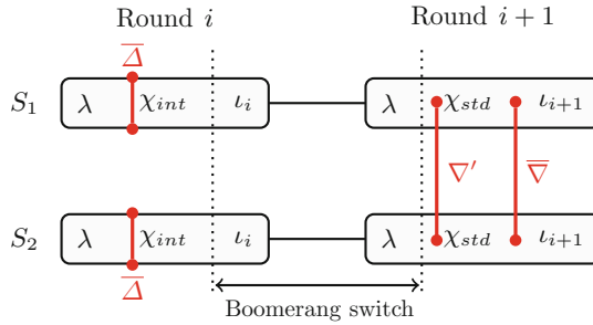
Fig. 2. The boomerang switch: middle of distinguishing structure where the differentials on the two halves of the primitive meet.
