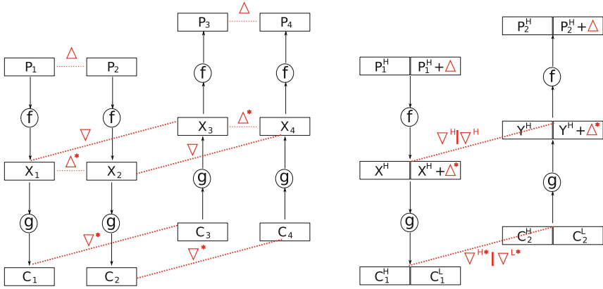
Fig. 1. The classical boomerangs (left). The internal differential boomerangs (right).
