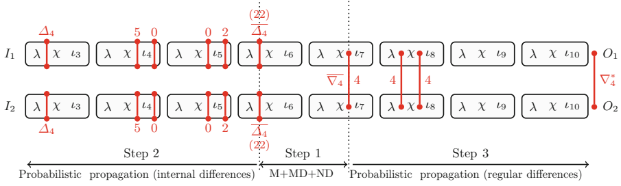
Fig. 3. Example of the internal boomerang distinguisher in the case of \text{Keccak-p}_{3,8} . In step 1, we first perform the matching (M), then the message modification (MD) and we use neutral bits (ND). We finish the construction of the pair of inputs (I_1, I_2) with the probabilistic propagations in Step 2 and 3.
