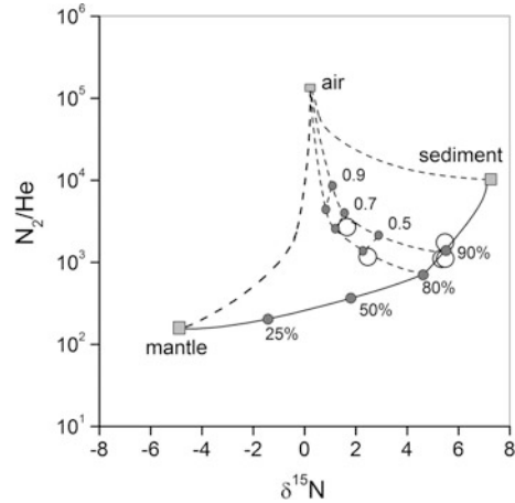
Fig. 6.11 \delta^{15}\text{N}_2 versus \text{N}_2/\text{He} binary diagram for gas samples from Copahue volcano. Boxes and mixing curves between the three end-members (Sediment, Mantle and Air) are from Sano et al. (2001) and Fischer et al. (2002)
