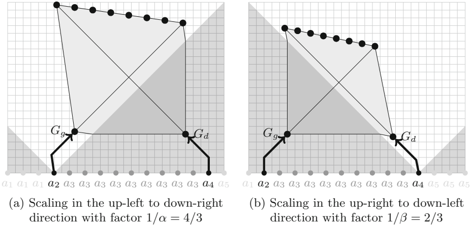
Fig. 4. Two scalings
