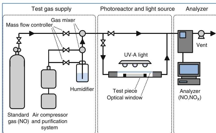
Fig. 9.4 Schematic of experimental apparatus (adapted from ISO 2007)
