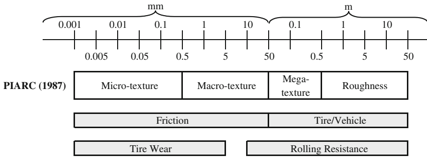
Fig. 6.2 Ranges in terms of texture wavelength and their influence on pavement-tire interactions. PIARC permanent international association of road congresses. Source adapted from Henry (2000) and Sandberg and Ejsmont (2002)
