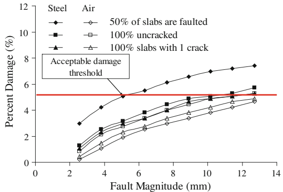
Fig. 6.13 Damage induced by different levels and counts of faulting
