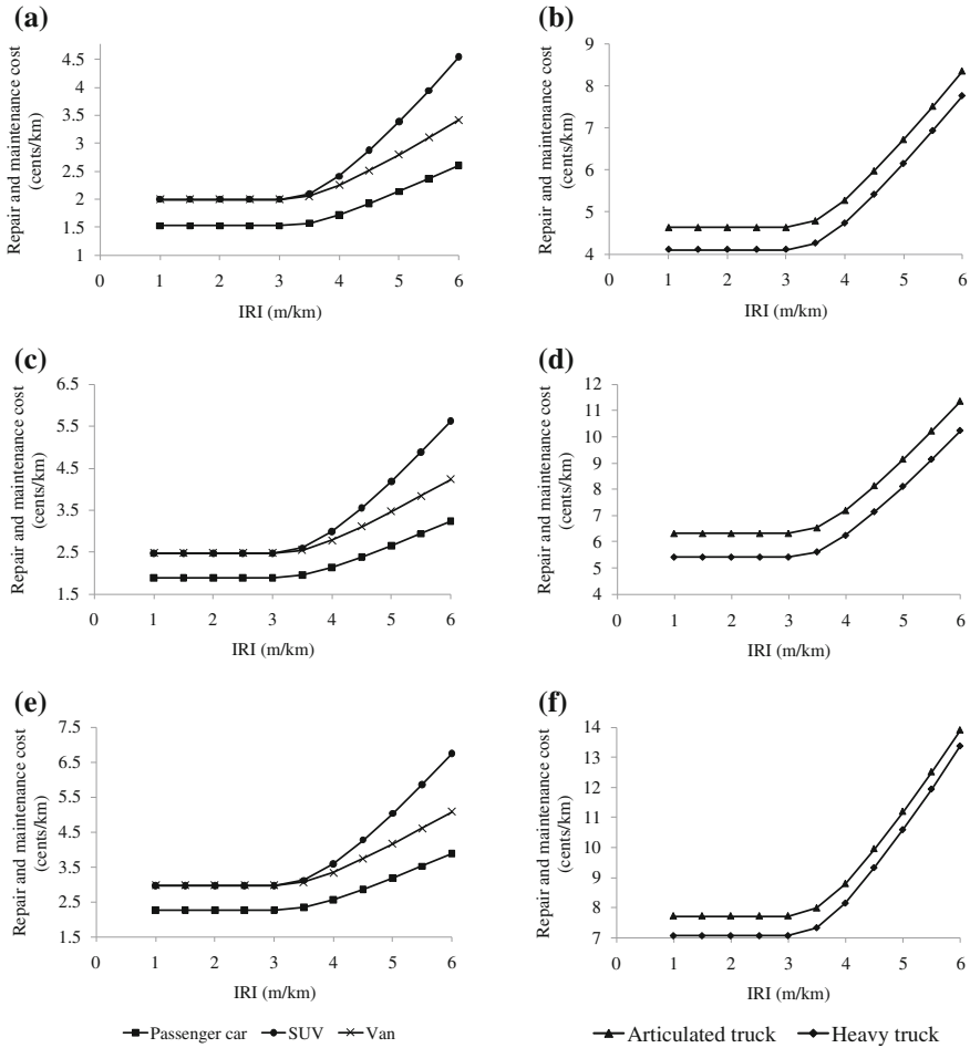
Fig. 6.21 Effect of roughness on repair and maintenance costs. a Light vehicles at 56 km/h (35 mph), b trucks at 56 km/h (35 mph), c light vehicles at 88 km/h (55 mph), d trucks at 88 km/h (55 mph), e light vehicles at 112 km/h (70 mph), f Trucks at 112 km/h (70 mph)
