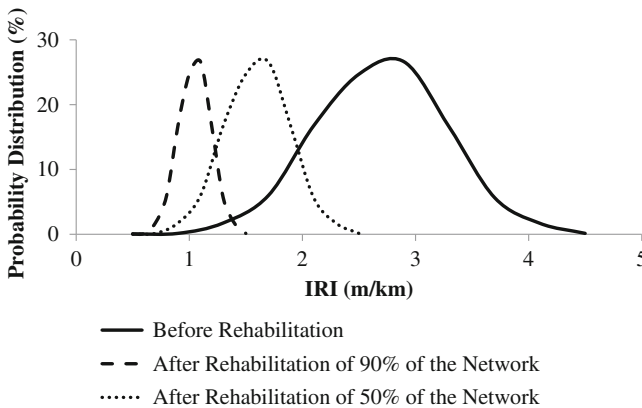
Fig. 6.27 Assumed roughness distribution for network pavement
