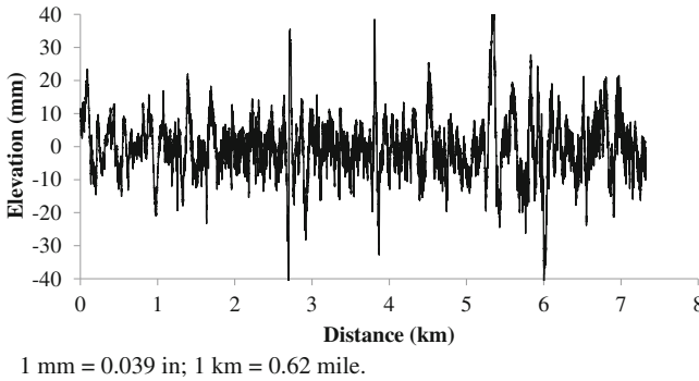
Fig. 6.22 Raw profile of the analysis section
