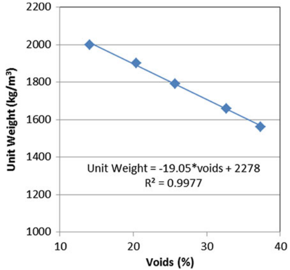
Fig. 8.1 Compaction density relationship for a single mixture
