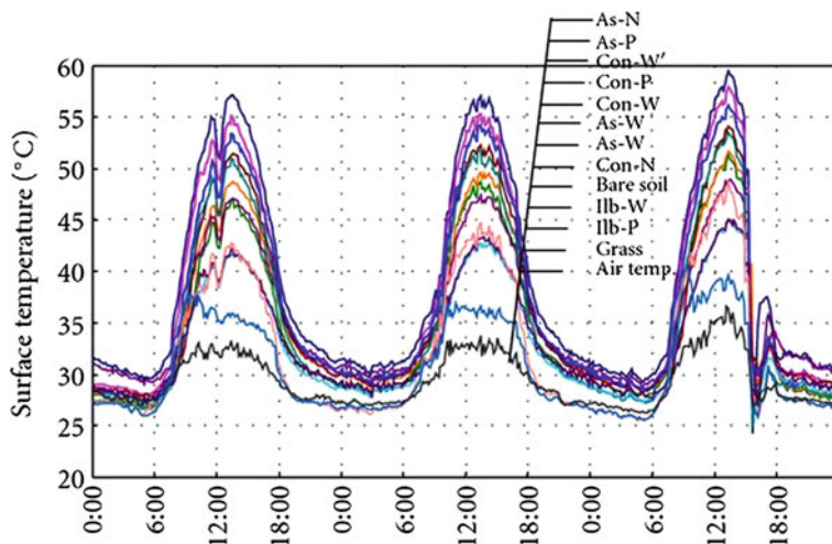
Fig. 18.20 Temperature in various experimental pavements (Takebayashi and Moriyama 2012). See Fig. 18.19 for explanation of codes
