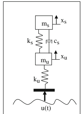
Fig. 6.8 Parameters for quarter-car vehicle model used. Source Chatti and Zaabar (2012)
