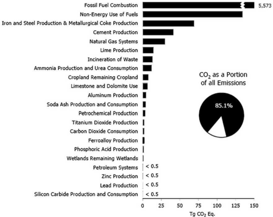
Fig. 16.3 Sources of US CO 2 equivalent emissions in 2008 (EPA 2010)
