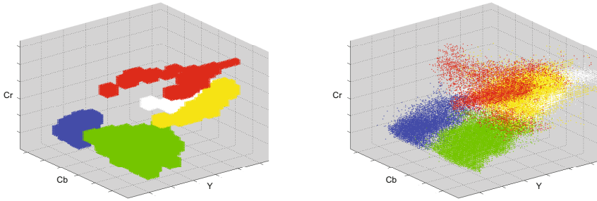
Fig. 2. Two examples of colour look-up tables generated for the training set of 50 images: a manually tuned LUT (left), created within the NUview utility using a point-and-click approach over the period of 1 hour; and an autonomously generated LUT (right), utilising k -means clustering over a subset of 30 training images and generated in less than 10 seconds.
