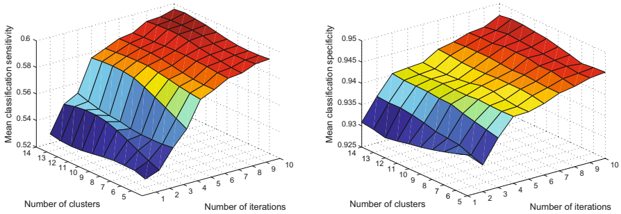
Fig. 4. Mean classification performance for colour look-up tables generated by k -means clustering, parameterised by both the number of clusters and clustering iteration count, presented in terms of sensitivity (left) and specificity (right). See Sec. 4.4 for definitions.
