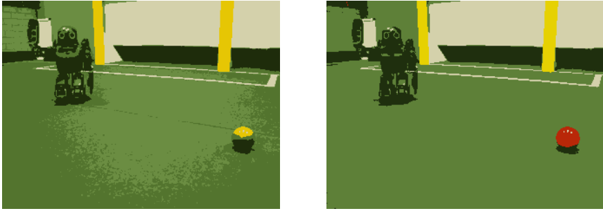
Fig. 1. An example of poor (left) versus good (right) quality colour image segmentation of a common RoboCup scenario. Segmentation was accomplished using the k -means algorithm ( k = 5 ) over RGB (left) and YC_bC_r (right) colour space representations [2].
