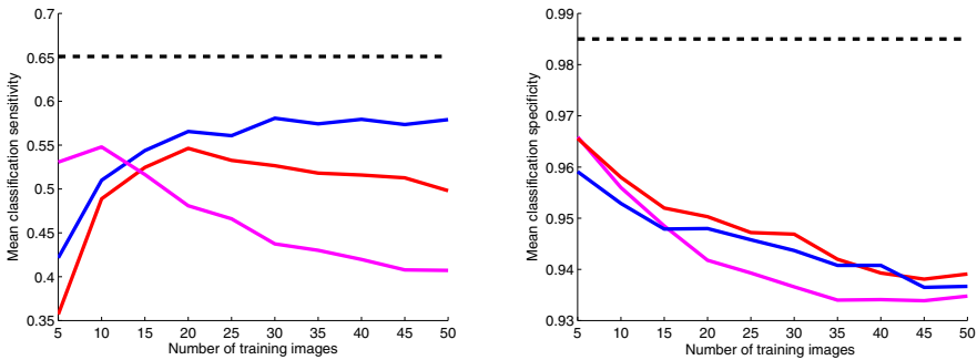
Fig. 3. Comparison of colour look-up table feature classification sensitivity (left) and specificity (right) as a function of the number of training images, for k -means (blue), expectation maximisation (red) and mean shift, utilising a flat kernel (magenta). The performance of a manually tuned LUT is indicated by the dashed lines. It is evident that k -means clustering yields the best classification sensitivity for most training set sizes, with comparatively little difference evident between the specificities of each method.
