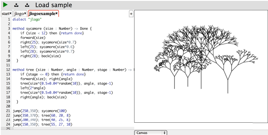
Fig. 2. A simple program in our Logo-like dialect and its output
