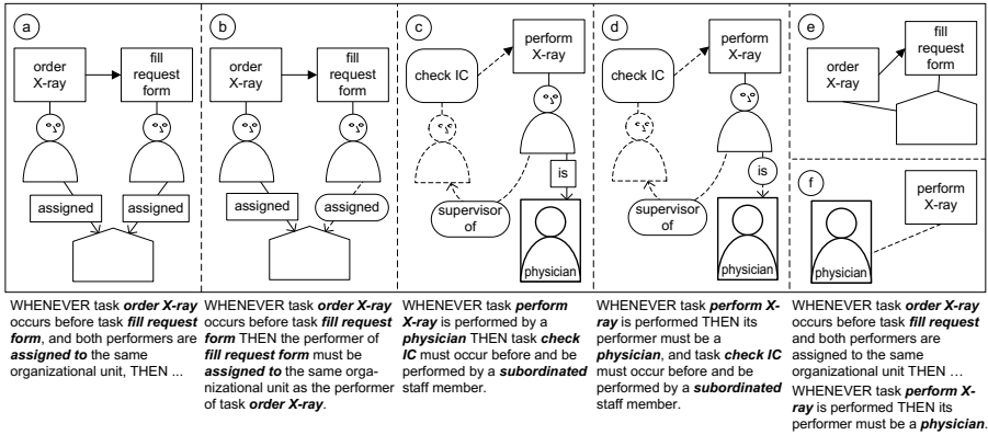
Fig. 11. Resource relations
