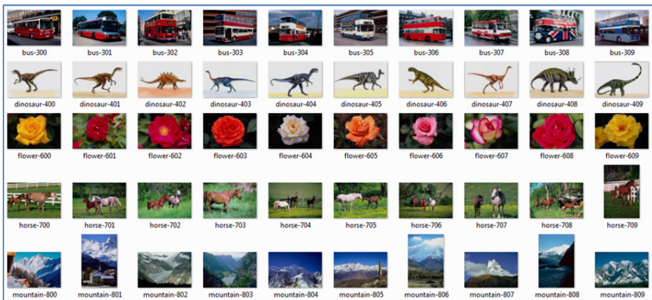
Fig. 3. Image Dataset
