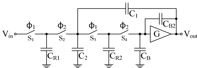
Fig. 1. Low-pass SC biquad filter in single-ended configuration
