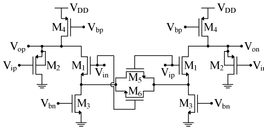
Fig. 4. Voltage-combiner amplifier with source degeneration
