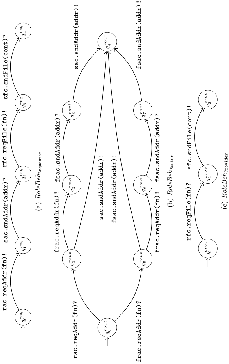
Fig. 5. Behaviors specifications
