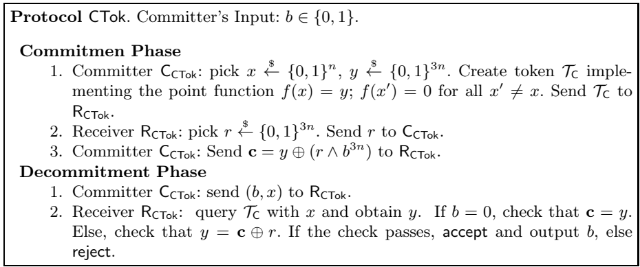
Fig. 3. CTok: Ideal Commitments in the \mathcal{F}_{\text{wrap}} model
