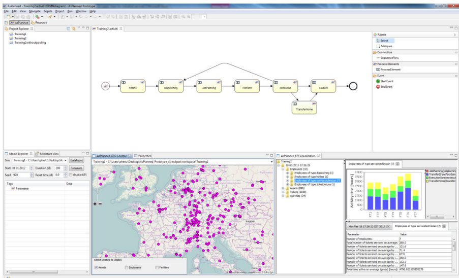
Fig. 1. General user interface of the AsPlanned Software
