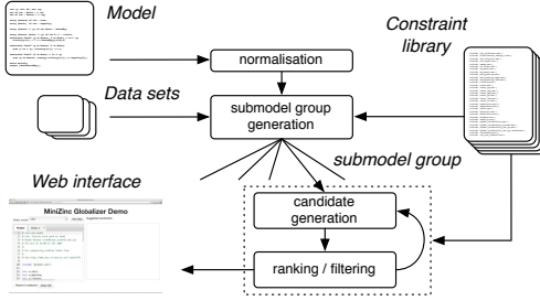
Fig. 2. An overview of model globalization
