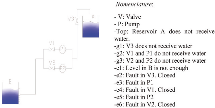
Fig. 2.1 Pumping station
