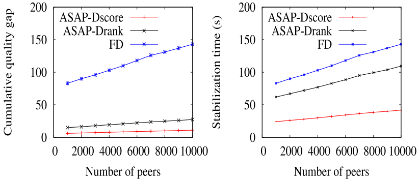
(a) Cumulative quality gap vs. Number of peers
