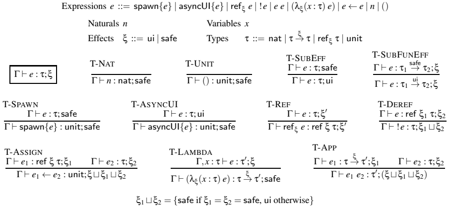
Fig. 1. \lambda_{\text{UI}} syntax for terms and types, and monomorphic type and effect system
