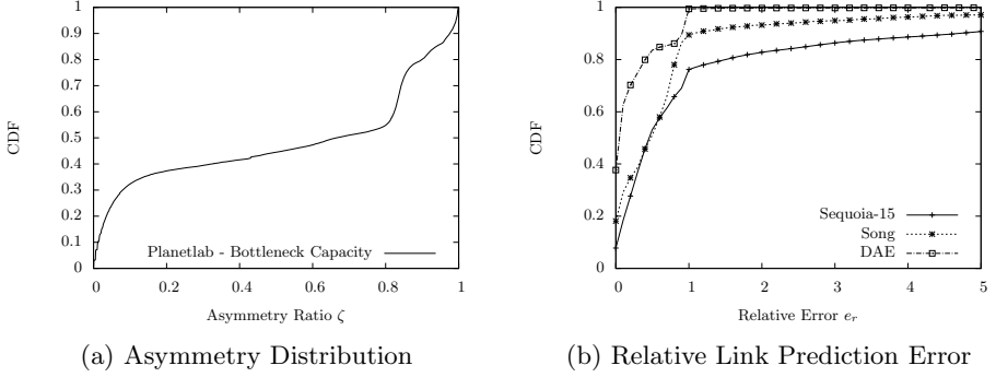
Fig. 5. PlanetLab Topology
