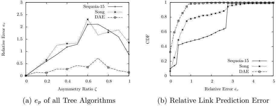
Fig. 6. Synthetic Dataset
