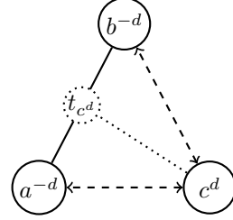
Fig. 3. Embedding Visualization
