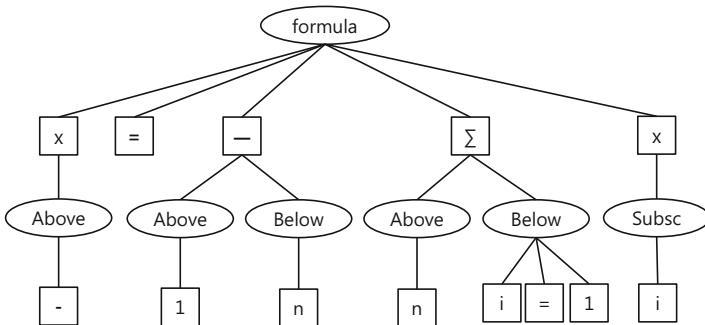
Fig. 2. Structure analysis process
