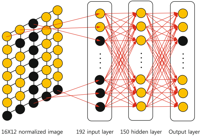
Fig. 8. Neural network structure of character recognition
