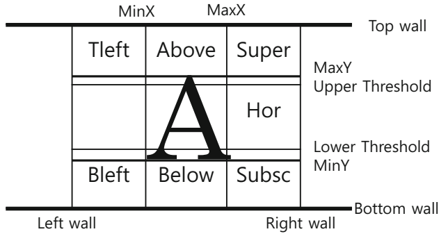
Fig. 1. Character region design
