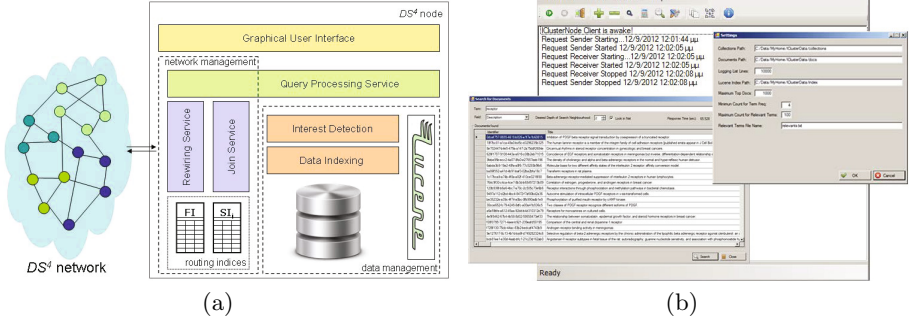
Fig. 1. (a) DS 4 node architecture and (b) GUI with results and settings screen
