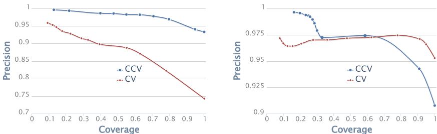
Fig. 2. Precision/Coverage graphs for CV and Binary CCV methods over the ScienceWISE (left) and MSH (right) collections
