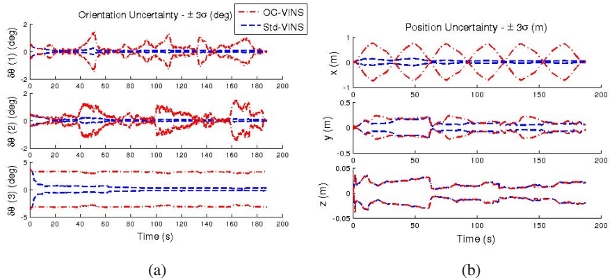
Fig. 4 Comparison of the estimated 3\sigma error bounds for attitude and position between Std-VINS and OC-VINS
