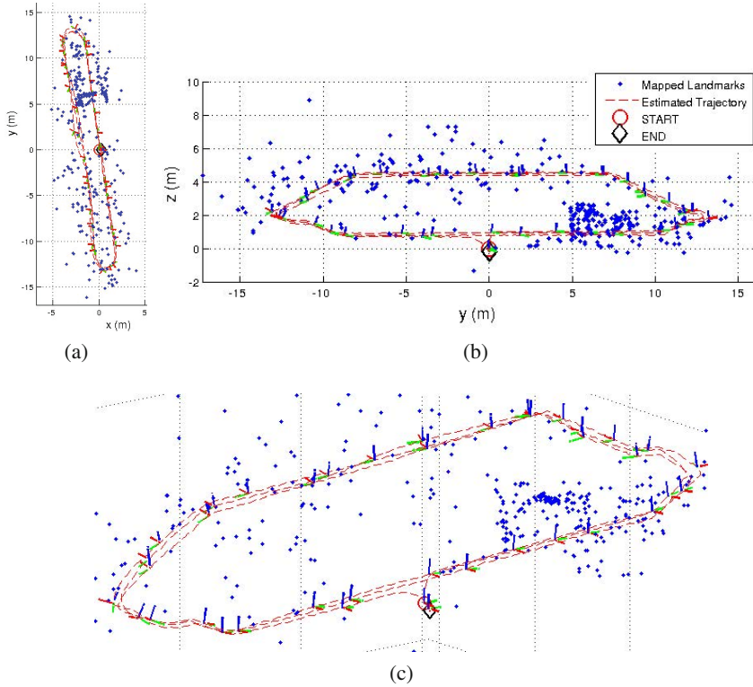
Fig. 3 The estimated 3D trajectory over the three traversals of the two floors of the building, along with the estimated positions of the mapped landmarks. (a) projection on the x and y axes, (b) projection on the y and z axes, (c) 3D view of the overall trajectory and estimated features.
