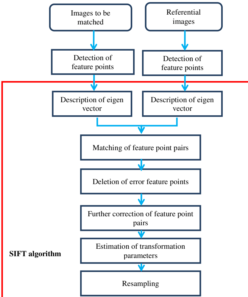
Fig. 3. Flow Chart of geometry fine correction
