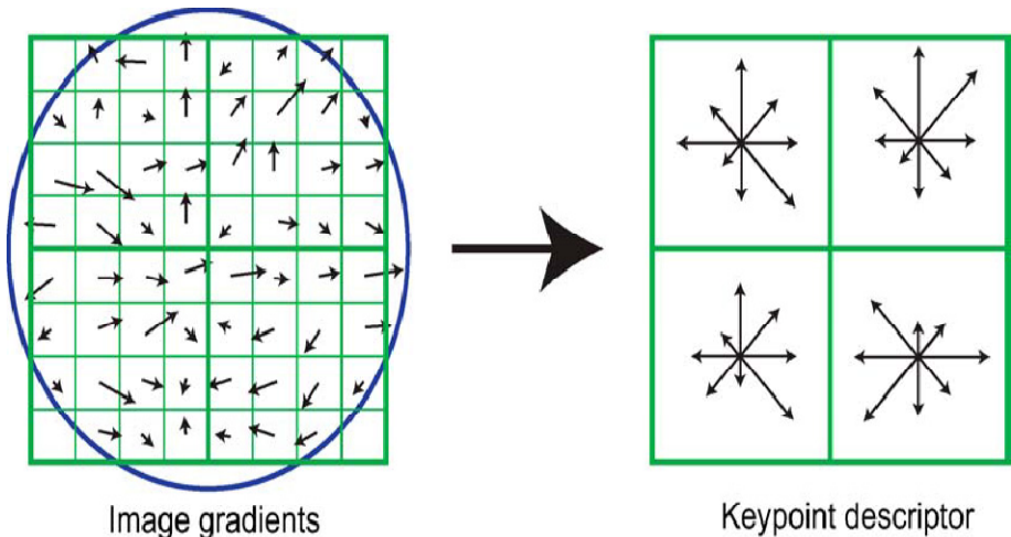
Fig. 2. Feature descriptor calculation process (Lowe, 2004)
