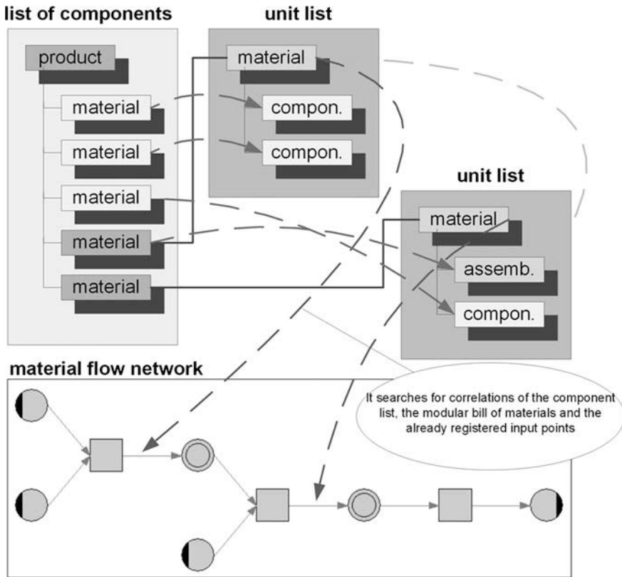
Fig. 5 Semi-automated production of output and connection places. Source Own
