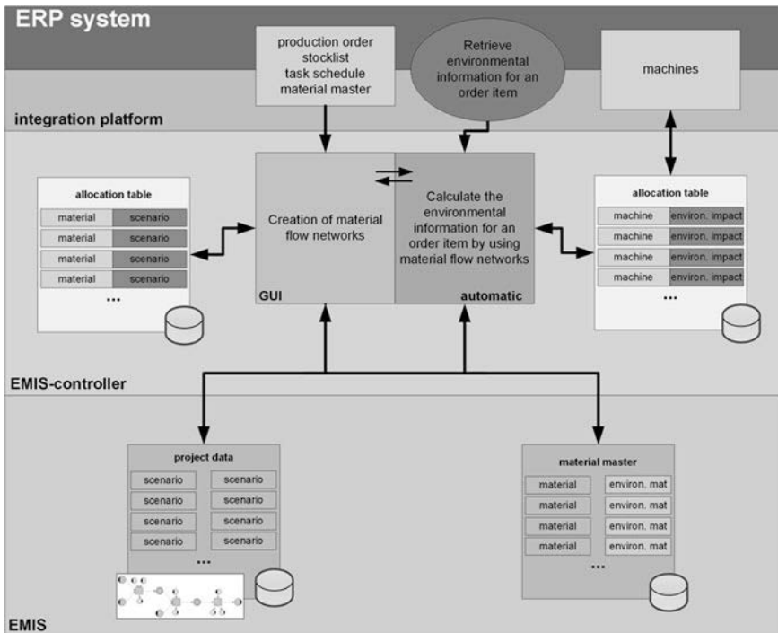
Fig. 1 Conceptual framework of integrated EMIS and ERP systems within the reference architecture of [10]. Source Own
