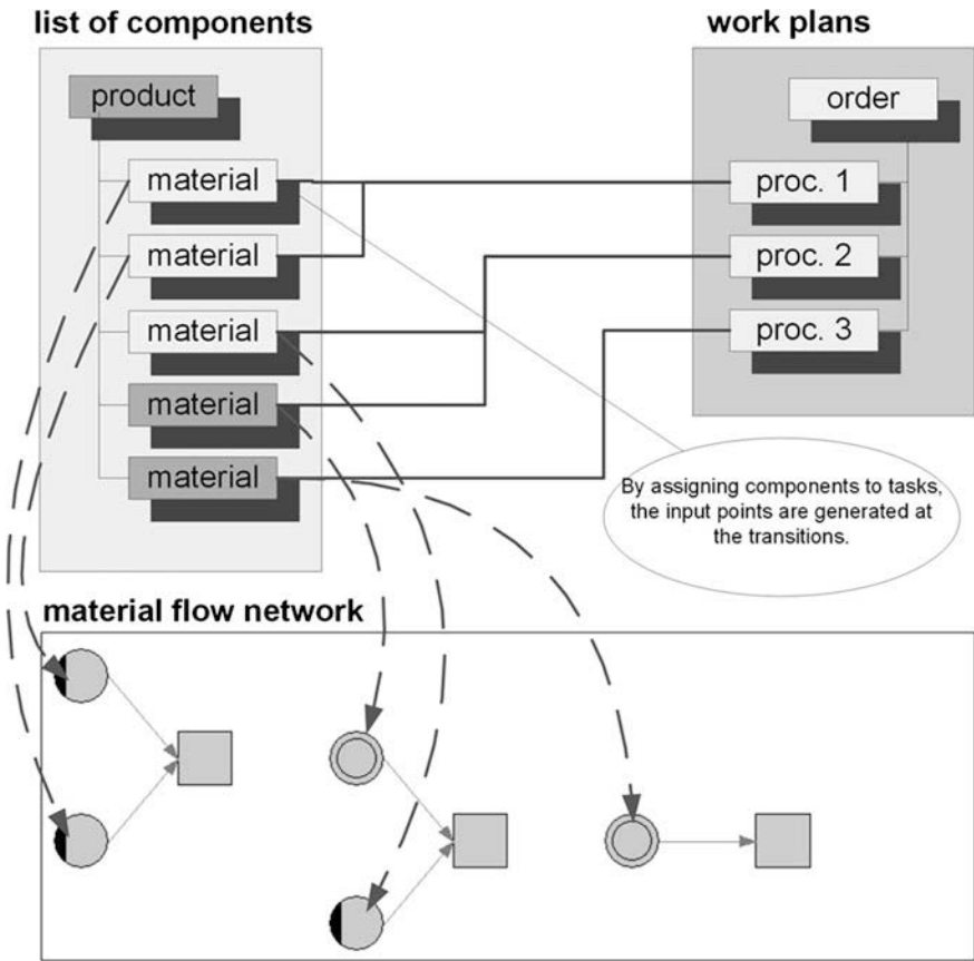
Fig. 4 Automated assignment of materials to the transitions as input. Source Own
