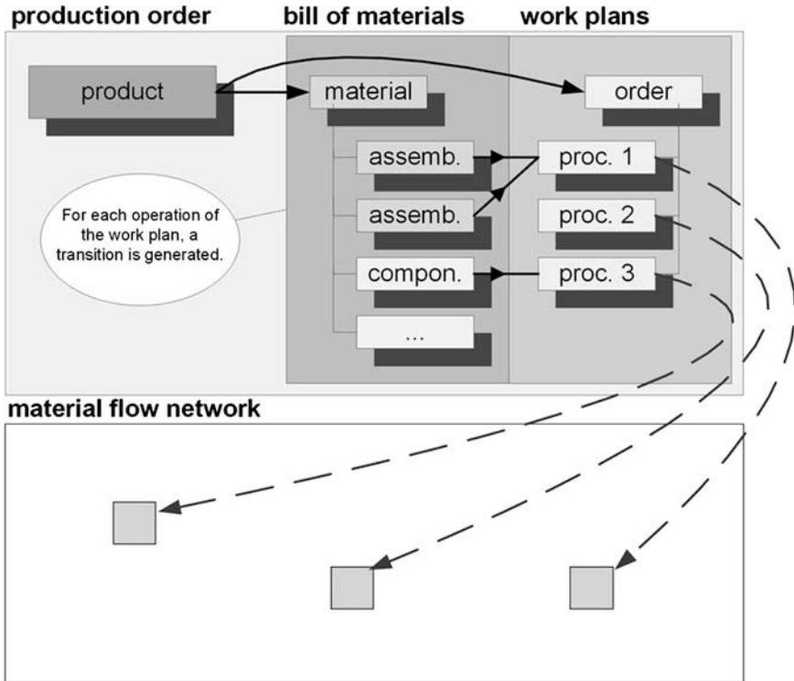
Fig. 3 Automated creation of transitions using operations from the production order. Source Own
