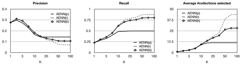
Fig. 4. Comparison of AENN collection selection strategies on the BTC\DBpedia collection
