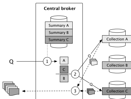
Fig. 1. Schematic overview of a typical broker-based distributed information retrieval system
