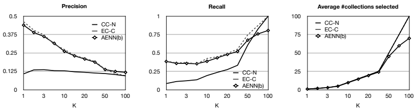
Fig. 5. Comparison of baseline and the AENN(b) collection selection strategies on DBpedia
