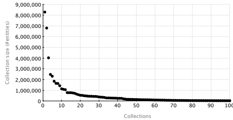
Fig. 3. Distribution of collection sizes in BTC-2009
