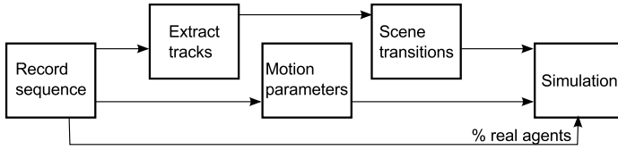
Fig. 1. Method workflow
