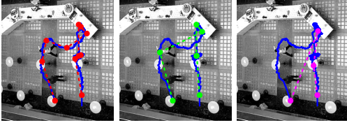
Fig. 2. The approximation of a real trajectory (in blue) for \kappa = 1 (red), \kappa = 10 (green) and \kappa = 100 (magenta). Note how a too small value of \kappa will introduce too many corners while the large value will miss some.
