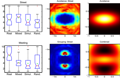
Fig. 4. Left: The results of the user study. The central red bar is the median score and the box extends from the 25-th to the 75-th percentile. The dashed lines go to the data points not considered as outliers (red cross). The green cross is the mean score. Center: The occupancy histogram for the Street sequence. Right: The energy terms after fitting to the histogram.
