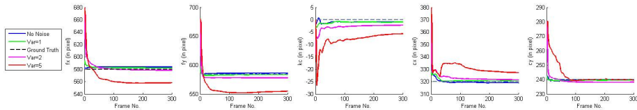
Fig. 4. Quantitative evaluation of our method for calibration on synthetic data, with respect to different level of noise, all intrinsic parameters are in pixels
