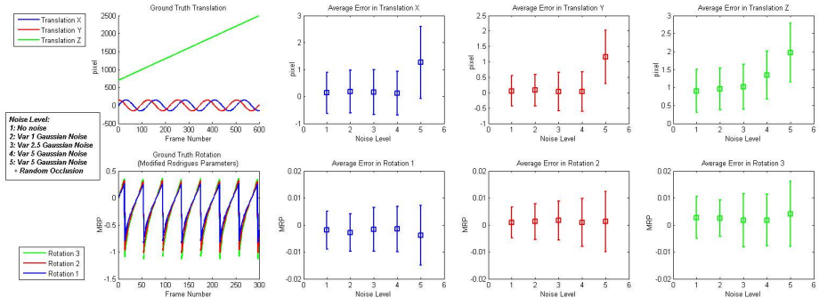
Fig. 3. Quantitative evaluation of the precision and robustness of our method for tracking 3D rigid object on synthetic data, with respect to different level of noise and occlusion. The error in translation is measured in pixel while rotation is measured in modified Rodrigues parameters.
