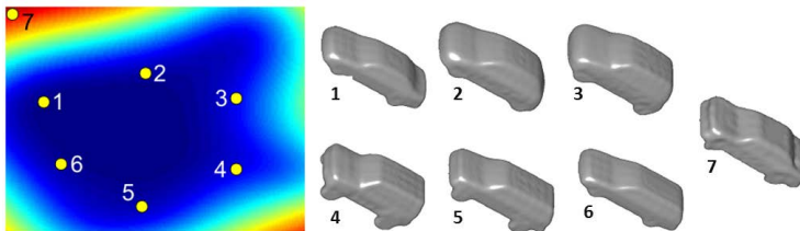
Fig. 9. Illustration of a 3D latent space of 3D car shapes: valid 3D car models (1~6) can be generated from the high-probability (blue) area in the latent space [9]
