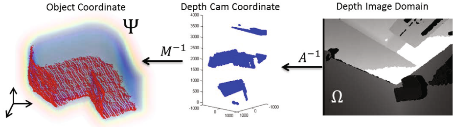
Fig. 1. Example of our back-projection formulation, from left to right: all pixels on the depth image are first unprojected into depth camera coordinate by intrinsic matrix A , then inverse transformed by extrinsic matrix M into the object coordinate, where the level-set embedding function is defined.
