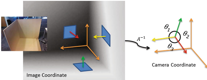
Fig. 6. Illustration of the criteria for the evaluation of intrinsic parameters: given a depth image of three orthogonal planes, we unproject all depth pixels from image coordinate to camera coordinate, then we compute the angle between the norms of the three orthogonal planes as criteria. If the intrinsic matrix is correctly recovered, the angle between the tree norm should all be 90^\circ .
