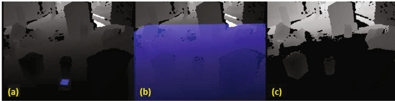
Fig. 7. Illustration of the ground plane removal step: a) fitting a plane patch to any part of the ground plane. b) Extend the plane patch. c) Ground plane is segmented out by removing all depth pixels that are close to the extended plane patch.
