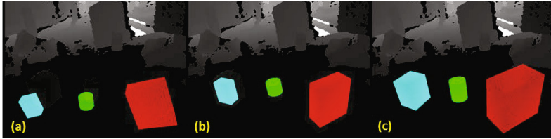
Fig. 8. Illustration of the model adaptation step: a) primitive models are initialized with arbitrary size; b) using our rigid 3D object tracking energy function, models are fitted into point cloud as rigid objects; c) shape adaptations energy function is used to simultaneously deform and track the primitives towards final fitting.
