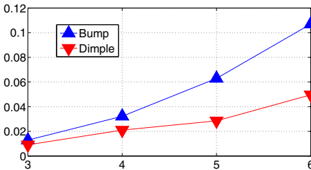
Fig. 2. Method evaluation for the synthetic AHC datasets. The ratio of the statistically significant mean shape surface voxels over the total number of surface voxels increases as the size of the synthetic distortion (bump or dimple) increases.
