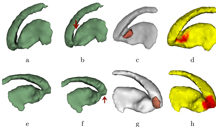
Fig. 3. Left (top) and Right (bottom) Striatum data sets. (a,e) Randomly selected examples of the left (a) and the right (e) striatum. (b,f) Left (b) and right (f) striatum shapes after applying shape deformations to the respective shapes shown in (a,e). (c,g) Mean (left and right) striatum shapes along with the averaged artificial deformation (red) (d,h) Mean (left and right) striatum shapes along with the respective p-value maps comparing distorted and undistorted data sets. Yellow indicates non-significant p-values. Red colors present a scale of FDR corrected p-values (below the threshold). Note that although the deformations and the extent of the deformed regions (pointed by arrows) are subtle, they were successfully detected by our algorithm.
