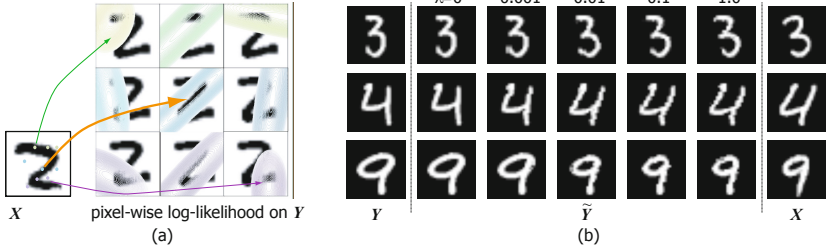
Fig. 3. (a) Pixel-wise log-likelihood for a pair of X and Y . For better visibility, only nine functions are plotted separately. (b) Matching results for different \lambda values.
