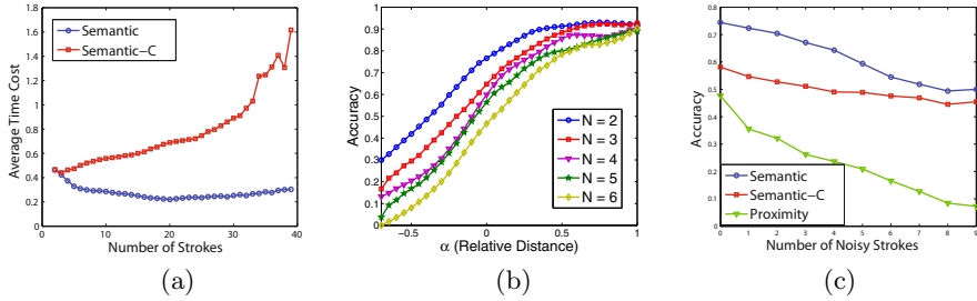
Fig. 10. (a) The average time cost for each newly drawn stroke. (b) Performance of the Semantic algorithm with different numbers of objects in the testing sketches. (c) Performance comparison under different numbers of noisy strokes.
