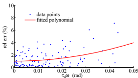
Fig. 3. Relative error on the parameters with respect to \tau_n \omega . The approximation seems to hold well until \tau_n \omega < 0.05 , which corresponds to error usually under 5%. Using correct camera parameters, this is large enough for any practical motion.
