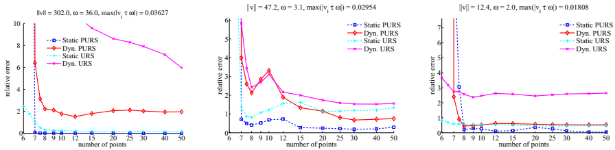
(a) Cube quickly rotating and translating, average exposure time. (b) Random points rotating slowly and translating quickly, long exposure time. (c) Random points slowly rotating and translating, long exposure time.
