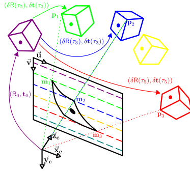
Fig. 2. The uniform rolling shutter camera model
