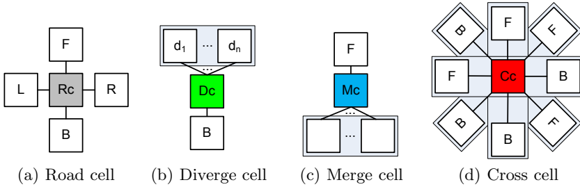
Fig. 3. Type of cells in an extended cellular lattice
