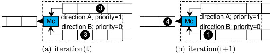
Fig. 4. Example of using the pass acceptance algorithm in a merge cell
