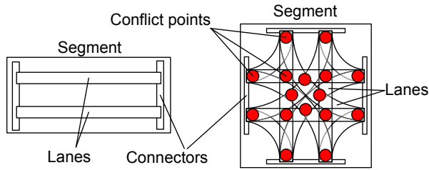
Fig. 2. Examples of the inner structure of segments
