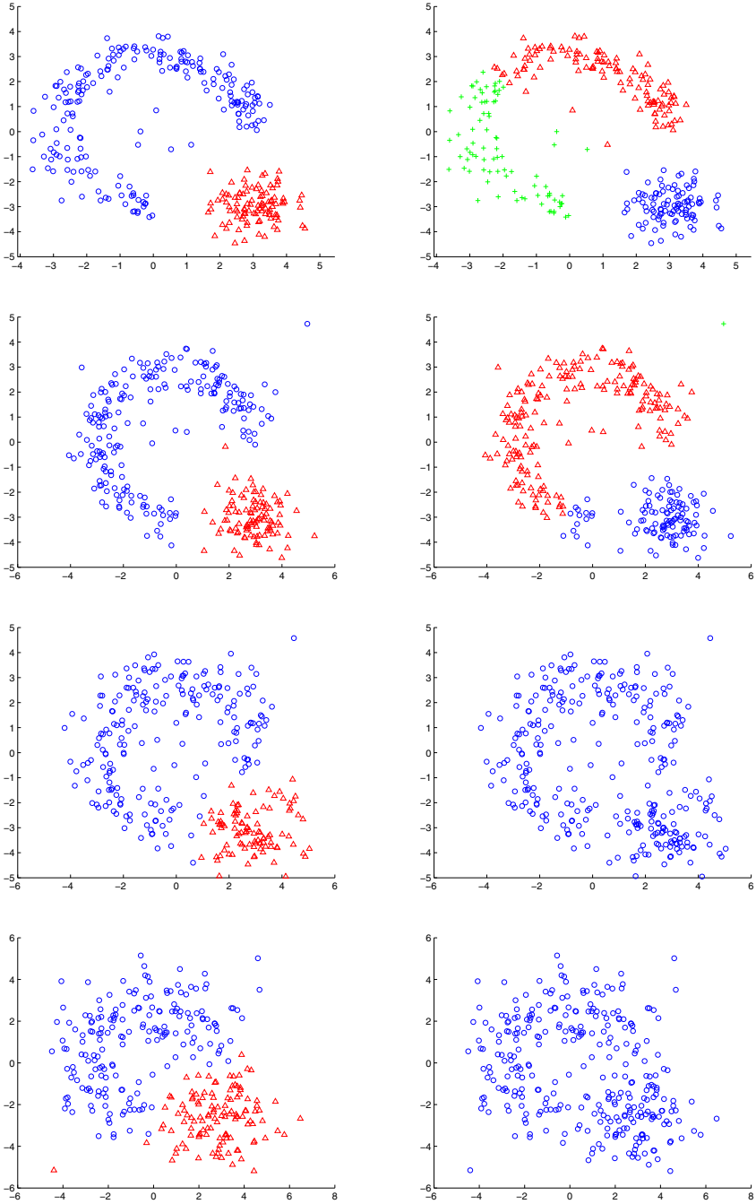
Fig. 3. Performance of Specplus (left) and DaSpec (right) for artificial data sets DS1, DS2, DS3, and DS4
