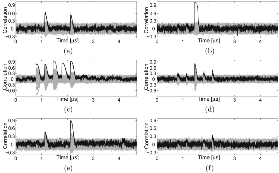
Fig. 7. BRAM version, collision attack results by S-box input model, (left) first-order (right) second-order: (a) and (b) Conventional , (c) and (d) First CT-RSA , (e) and (f) Second CT-RSA profiles, each using 1 000 000 traces
