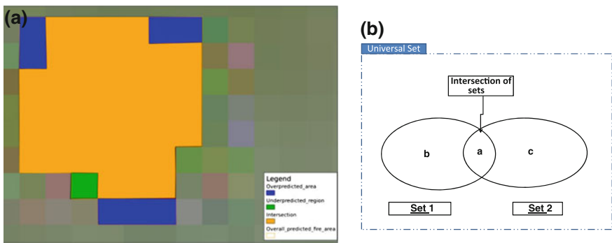
Fig. 13 Illustrations of the components of Sorenson coefficient for validation of fire spread model
