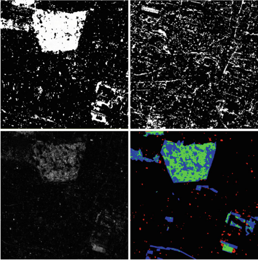
Fig. 3 Same detail as Fig. 1. ( Top ) IR-MAD variate 1 and 2, White = change; ( Bottom left ) result of MAD algorithm: Chi-square image, lighter = higher probability of change; ( Bottom right ) overlay of resulting IR-MAD binary map and manual measurement (legend: see Fig. 2)
