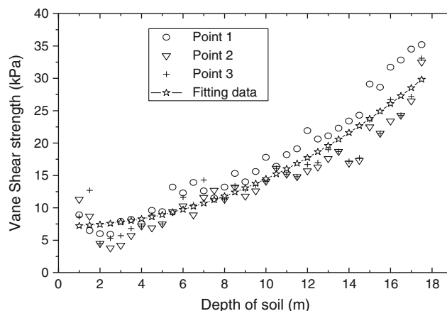
Fig. 2 Relationship of test data and fitting data
