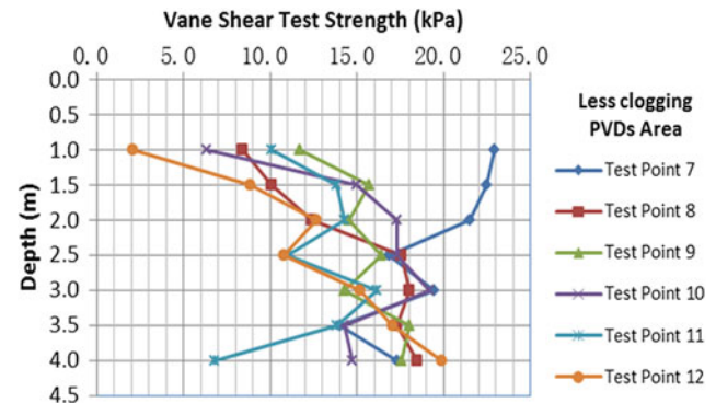
Fig. 8 Vane shear test strength of less clogging PVDs area
