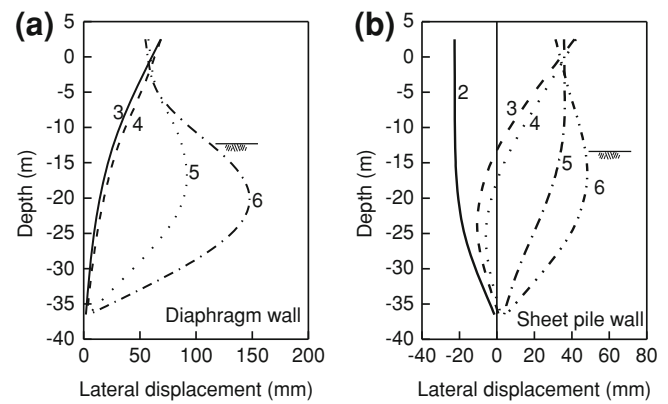
Fig. 3 Lateral displacement of retaining wall
