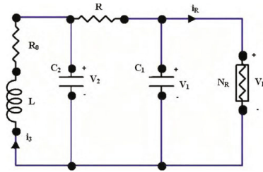
Fig. 1. Classical Chua's circuit
