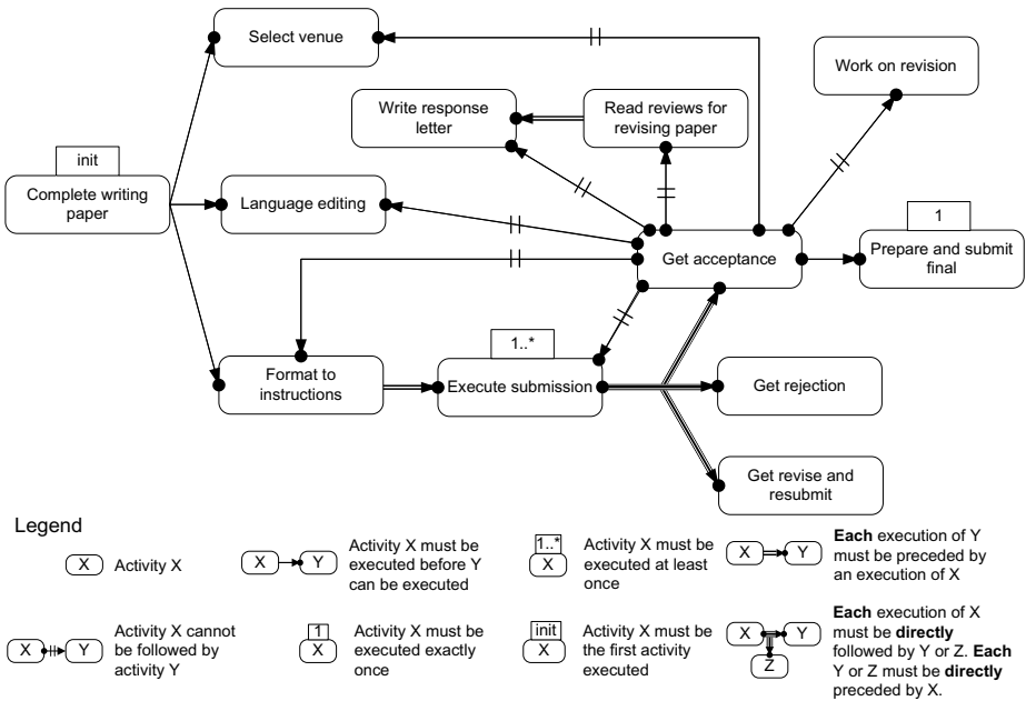
Fig. 3. Example of a flat model
