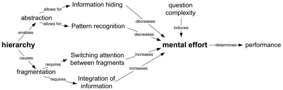
Fig. 6. Framework for assessing hierarchy, adapted from [17]
