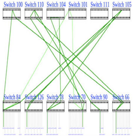
Fig. 5. Link utilization of scatter-allgather algorithm
