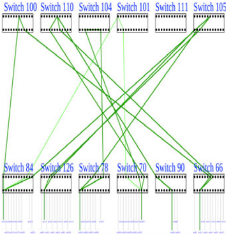
Fig. 4. Link utilization of binomial algorithm
