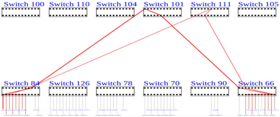
Fig. 6. INAM depicting the communication pattern using LU benchmark
