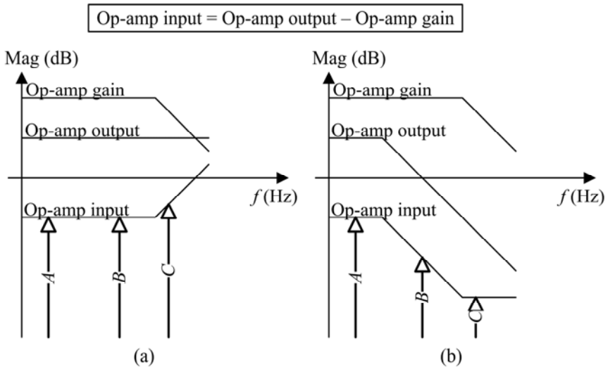
Fig. 3. Illustration of the pre-filtering effect of an op-amp based CSF. (a) The case with an op-amp based TIA, and (b) the case with an op-amp based CSF.
