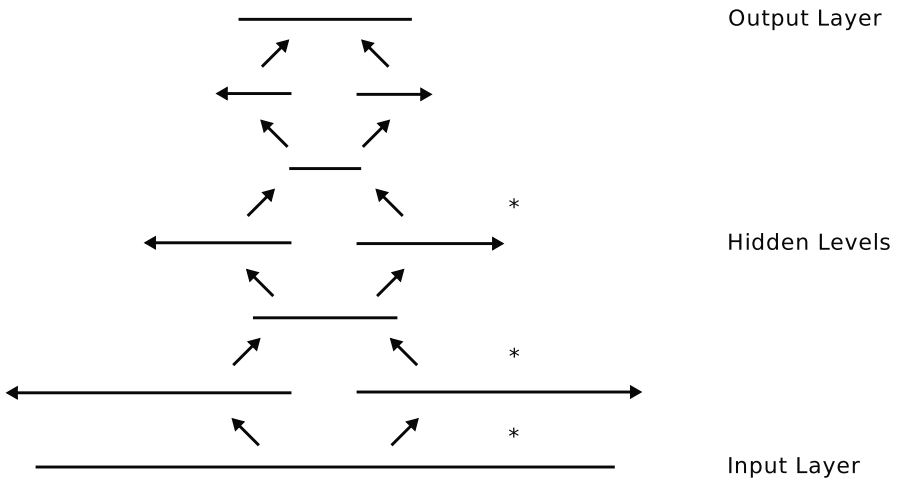
Fig. 9.3 Information flow through a multidirectional HSRNN. Each hidden level consists of two recurrent layers scanning in opposite directions. Each pair of hidden levels is separated by a feedforward layer (with no scanning arrow). Subsampling is carried out at the places indicated with a ‘*’. Note that the outputs of the final hidden level are neither subsampled nor passed through a feedforward layer before being fed to the output layer.
