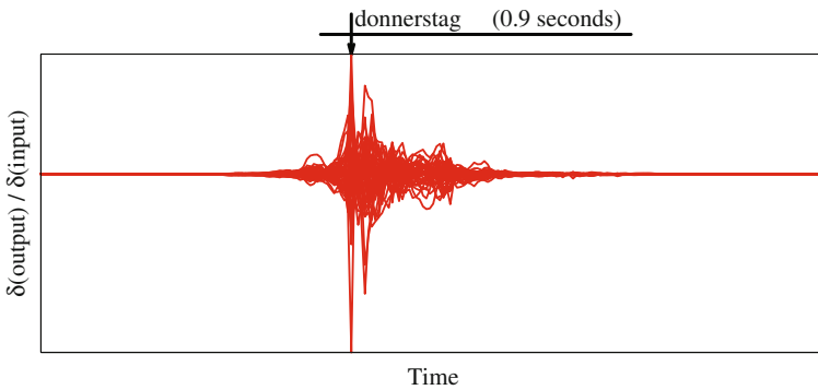
Fig. 7.8 Sequential Jacobian for keyword spotting on Verbmobil
