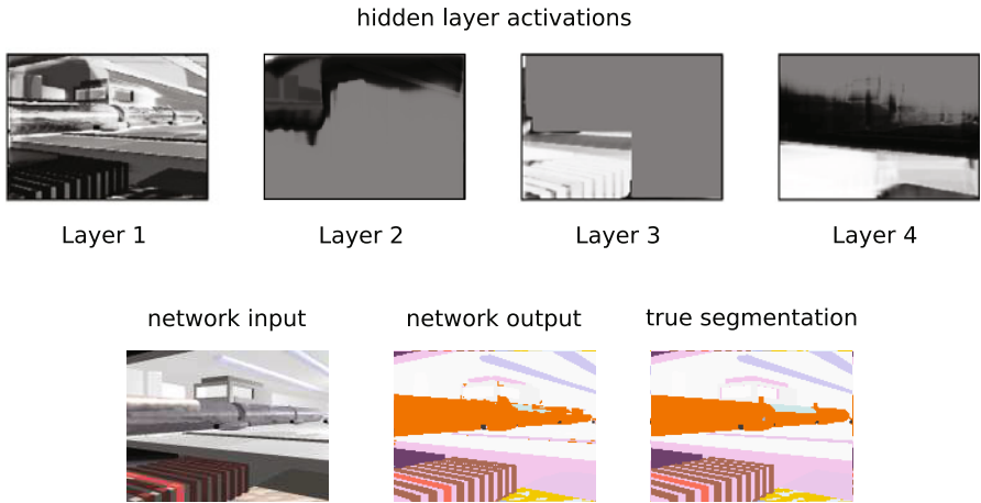
Fig. 8.9 MDRNN applied to an image from the Air Freight database. The hidden layer activations display one frame from each of the layers. A common behaviour is to ‘mask off’ parts of the image, exhibited here by layers 2 and 3.
