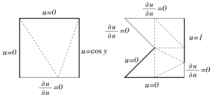
Fig. 8.7. Example 8.9. Domains and initial coarse grids. Black lines : Dirichlet boundary conditions, grey lines : Neumann boundary conditions. Left : Example 8.9a, unique solution exists. Right : Example 8.9b, no solution exists.
