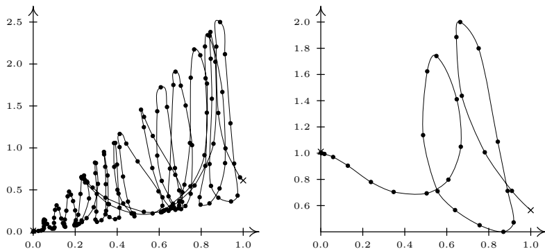
Fig. 5.1. Example 5.1. Left: unspecific embedding (5.3). Right: problem-oriented embedding (5.4).
