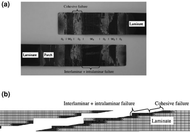
Fig. 35 Type B failure for a 3° scarf angle repair: experimental fracture surfaces (a) and FE prediction (distorted image for a clear visualization) (b) (Campilho et al. 2009a)
