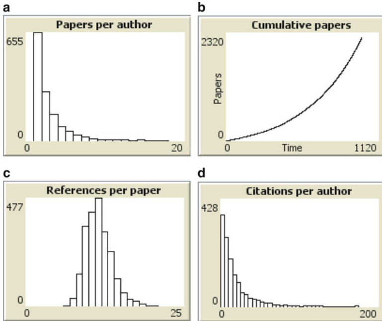
Fig. 4.6 Numerical relationships in a sample run of Gilbert’s simulation. Figure 4.6 shows the approximation of Lotka’s law. The figures are taken from Gilbert’s NetLogo replication of his original model, freely available at http://www.openabm.org/model-archive/ssas
