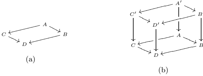
Fig. 4. A pushout square (a) and a commutative cube (b)
