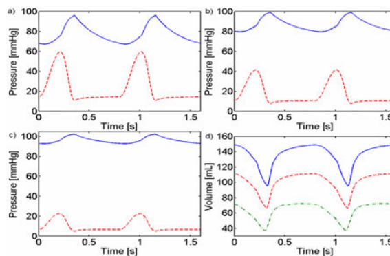
Fig. 5 a) LV pressure and aortic pressure at 7800-11250 rpm, b) LV pressure and aortic pressure at 9300-11250 rpm, c) LV pressure and aortic pressure at 10300-11250 rpm, (- -LV pressure, -aortic pressure), d) LV volume (- 7800-11250 rpm, --9300-11250 rpm, - .10300-11250 rpm)
