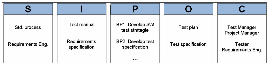
Fig. 1. Example “SIPOC”
