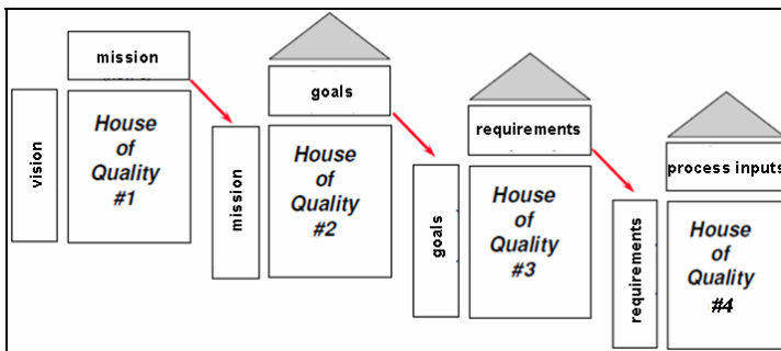
Fig. 6. Example “QFD”
