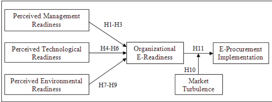
Fig. 1. Theoretical Framework
