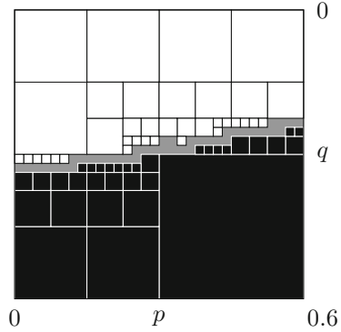
Fig. 1. Dividing the parameter space into regions in the Zeroconf example
